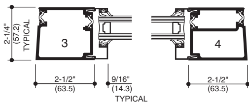
LOCK STILE
